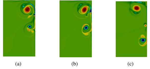
FIG. 13: Vorticity plots for oblique wall dipole collision at angle of 30^\circ and time t = 0.7 for no slip walls and for slip-lengths \zeta = 0.002, 0.01 when Re = 2500 . Contours are shown in the subdomain 0.2 \leq x \leq 1, -0.4 \leq y \leq 1 in the vicinity of the collision. (a) No slip, (b) \zeta = 0.002 and (c) \zeta = 0.01 .
