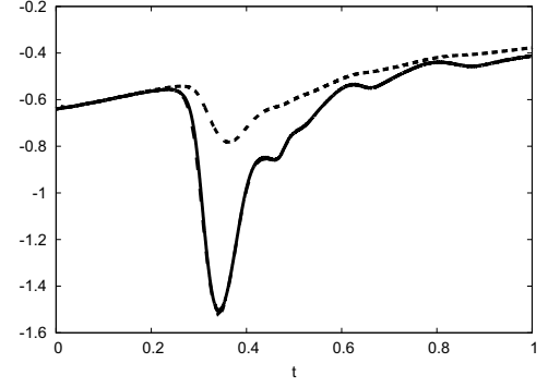
FIG. 26: Relationship between the energy dissipation and the enstrophy in equation (37) for dipole wall collision with slip length \zeta = 0.004 and Re = 2500 . Shown are the left side of the equation (37) (dashed line), the right side (solid line) and the right side of equation (38) (dotted line).
