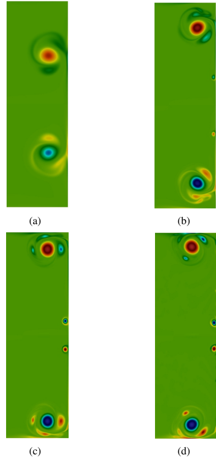
FIG. 8: Plots of vorticity for normal wall dipole collision with \zeta = 0.01 at t = 1 for various Reynolds numbers. Contours are shown in the subdomain 0.4 \leq x \leq 1, -1 \leq y \leq 1 in the vicinity of the collision. (a) Re = 1252 , (b) Re = 5000 , (c) Re = 7500 and (d) Re = 10000 .
