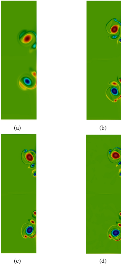
FIG. 7: Plots of vorticity for normal wall dipole collision with \zeta = 0.01 at t = 0.6 for various Reynolds numbers. Contours are shown in the subdomain 0.4 \leq x \leq 1, -1 \leq y \leq 1 in the vicinity of the collision. (a) Re = 1252 , (b) Re = 5000 , (c) Re = 7500 and (d) Re = 10000 .
