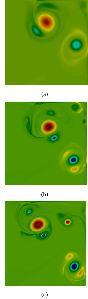
FIG. 17: Vorticity fields of dipole wall collision at an angle of 30^\circ at time t = 1.5 with slip length \zeta = 0.002 and (a) Re = 2500 , (b) Re = 5000 and (c) Re = 7500 . Contours are shown in the subdomain 0 \leq x \leq 1, 0 \leq y \leq 1 in the vicinity of the collision.
