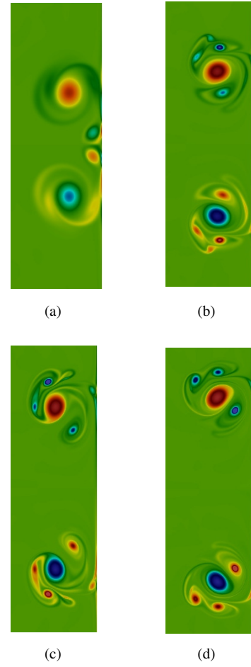
FIG. 6: Plots of vorticity for normal wall dipole collision at \zeta = 0.002 and t = 1 for various Reynolds numbers. Contours are shown in the subdomain 0.5 \leq x \leq 1, -0.8 \leq y \leq 0.8 in the vicinity of the collision. (a) Re = 1252 , (b) Re = 5000 , (c) Re = 7500 and (d) Re = 10000 .
